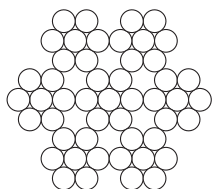
6x7+WS
