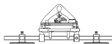
Ventosa a 2 piastre Two suction pads
